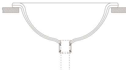
Drop-In Installation shown without Overflow
