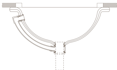
Undermount Installation shown with Overflow
