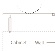
Front: Two Part Leveling Leg Back: Surface Clips
