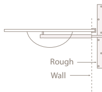
Front: In-wall Mount Back: Recessed U-Channel
