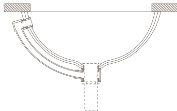
Undermount Installation with Overflow Shown with Vitraform Countertop
